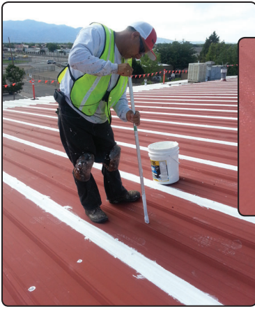
Sealing fasteners with Apoc 264
