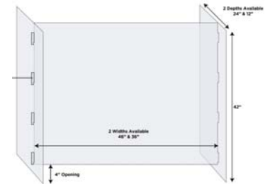
Protection Barrier
