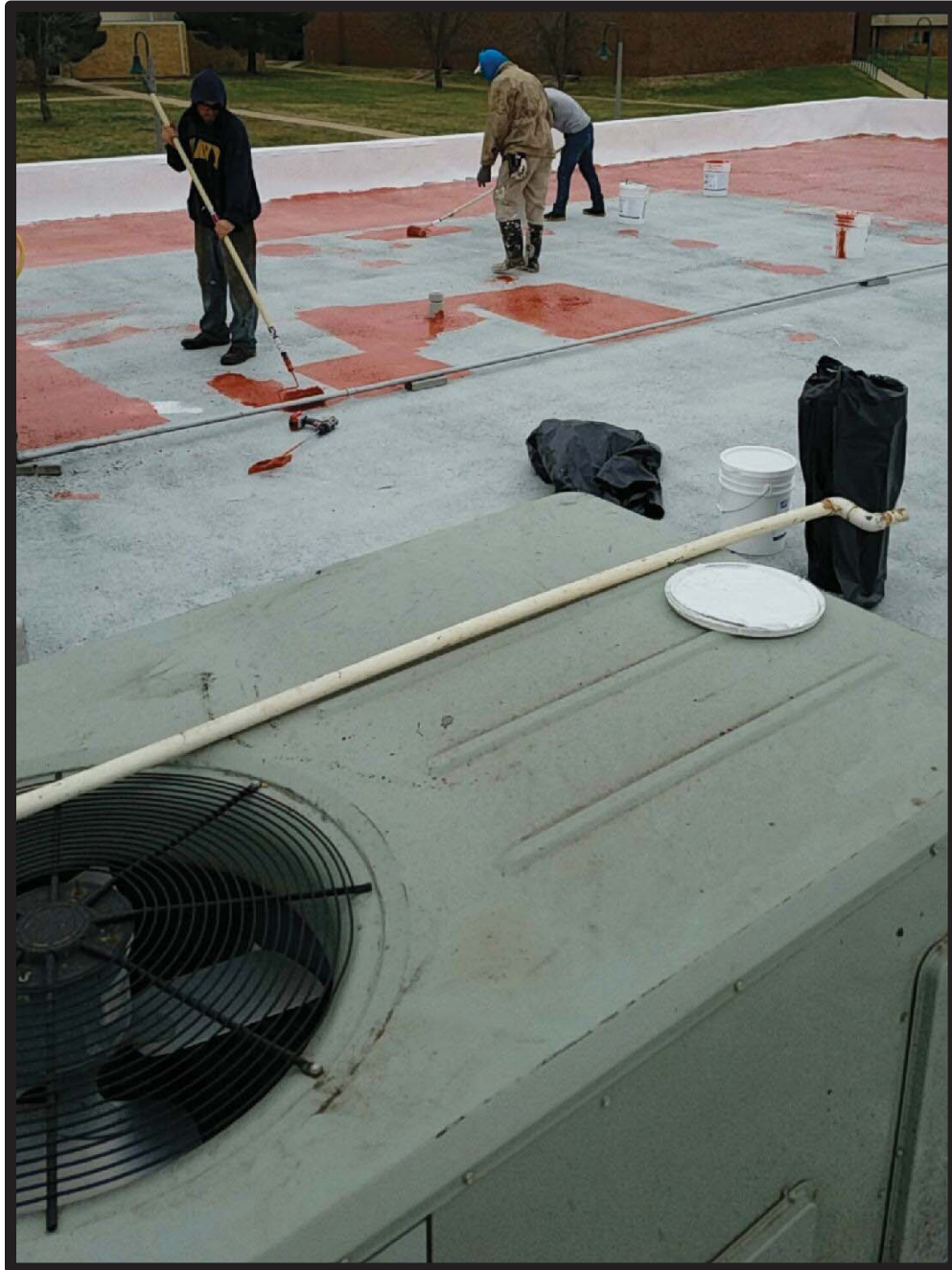
Prime entire roof area with Bleed Block (gray) to prepare for silicone coats. (Only needed on existing asphaltic based roofing systems)
