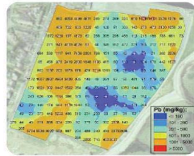
Concentration Contour Map of Pb in Soil
