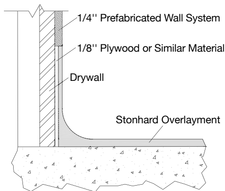
COVE BASE DETAIL with Pre-fabricated Wall System
