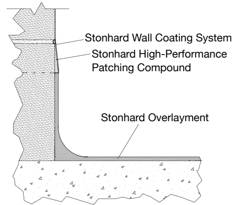
GMP COVE BASE DETAIL WITH CMU BLOCK
