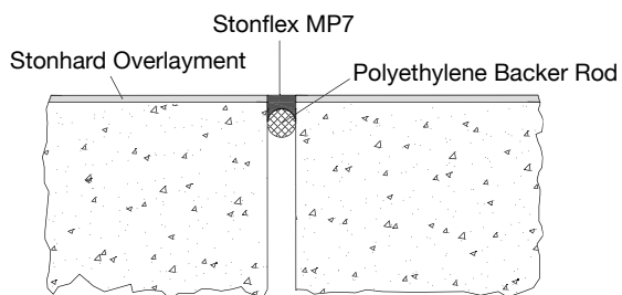
JOINT EXPANSION / ISOLATION JOINT DETAIL
