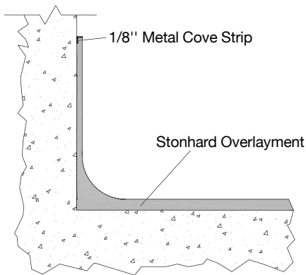
COVE BASE DETAIL WITH COVE STRIP
