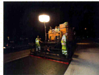
Microsurfacing
