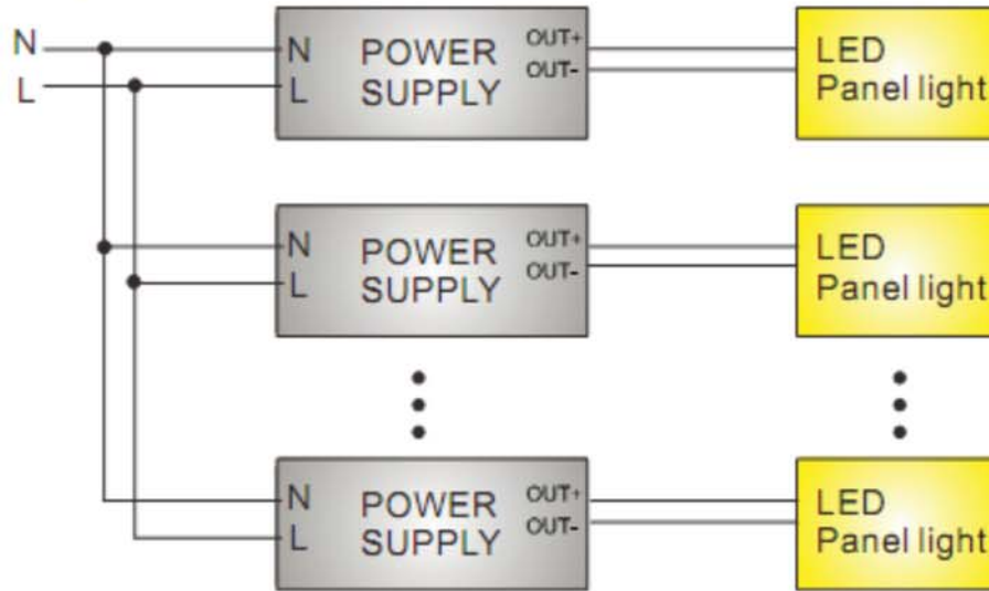
A. Wiring of the panel light with non-dimmable driver
