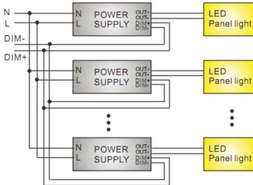
B. Wiring of the panel light with 0-10V dimmable driver
