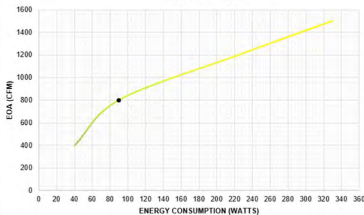
EQUIVALENT OUTDOOR AIRFLOW VS ENERGY CONSUMPTION
