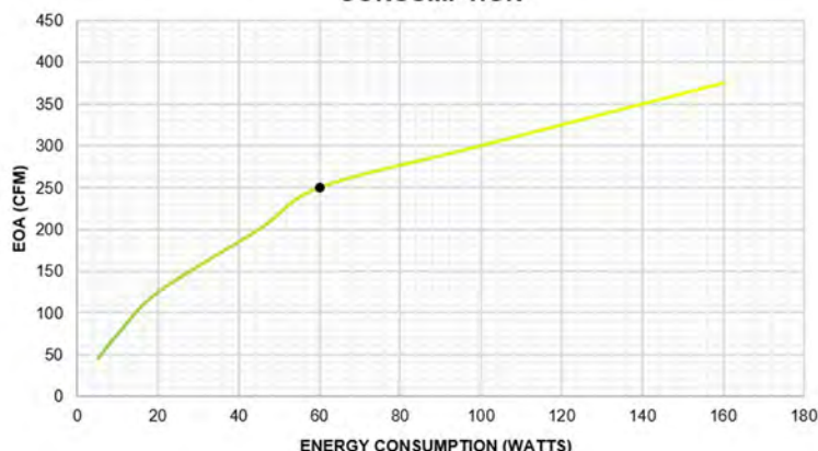
EQUIVALENT OUTDOOR AIRFLOW VS ENERGY CONSUMPTION
