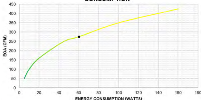
EQUIVALENT OUTDOOR AIRFLOW VS ENERGY CONSUMPTION
